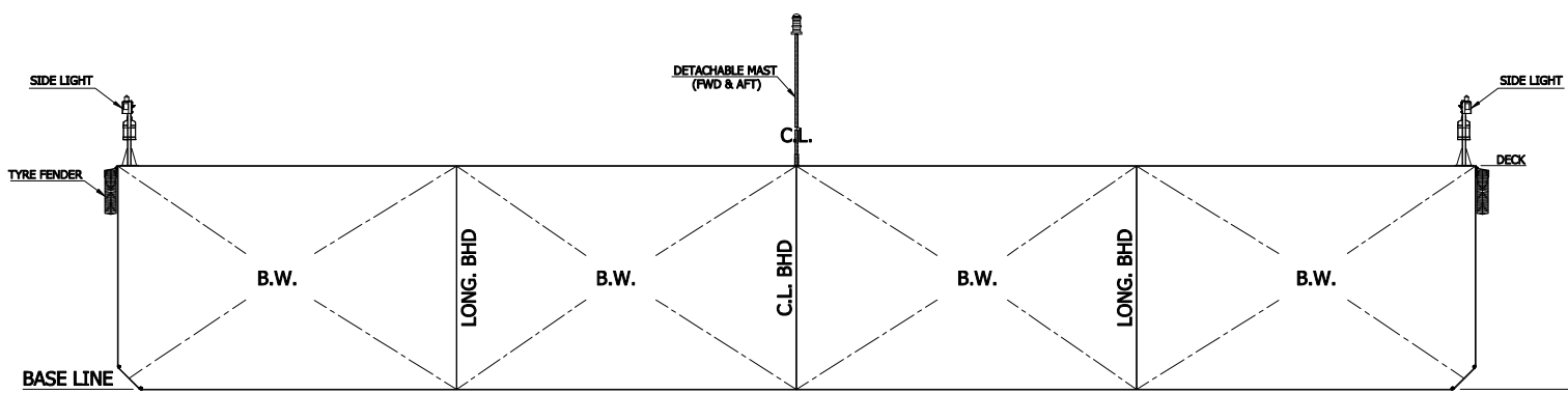
SECTIONAL VIEW
